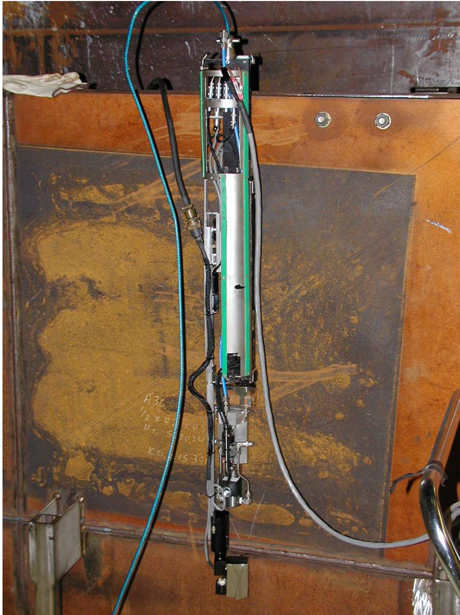
Figure 2-5 Modified Wall Crawler on Tank Mockup Wall
