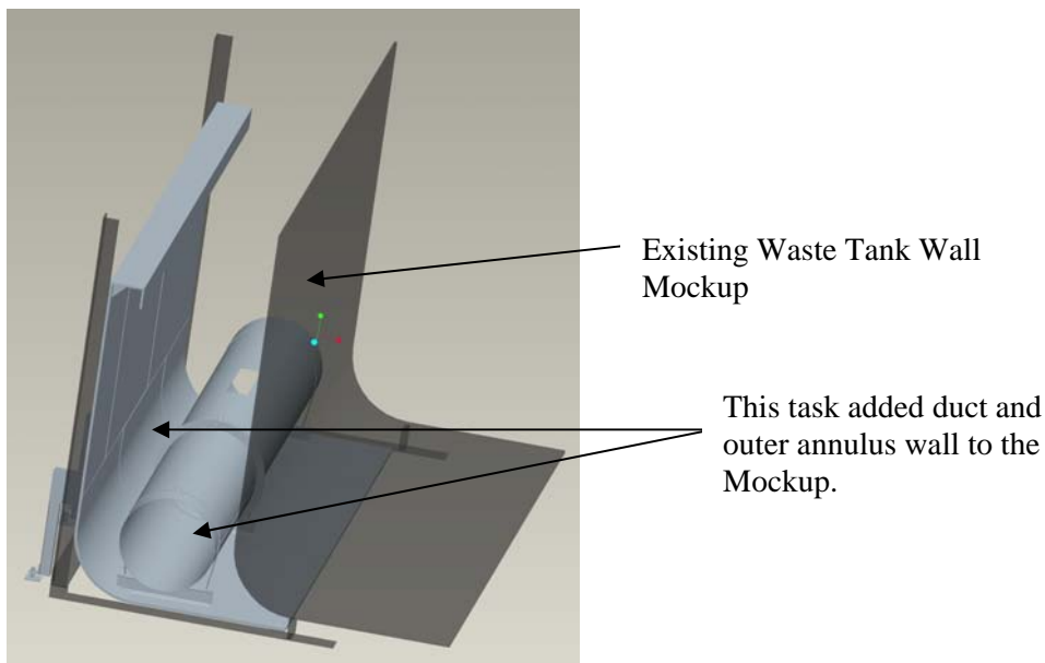
Figure 2-1 723-A Annulus Mockup Modification
