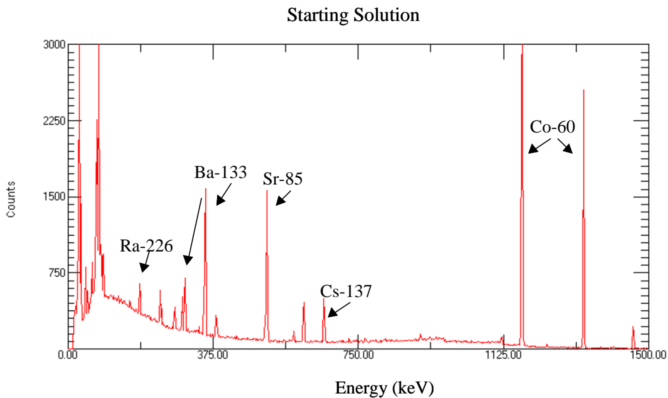
Figure 4 Gamma energy spectrum for the radionuclide control solution used in the low-level radionuclide exposures with the SPME fibers.
