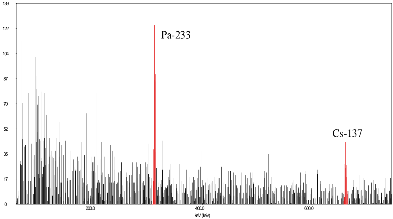
Figure 1 Gamma X-ray spectrum for the bag of five SPME fibers, which contained one of each SPME fiber from the pH 2 exposures.
