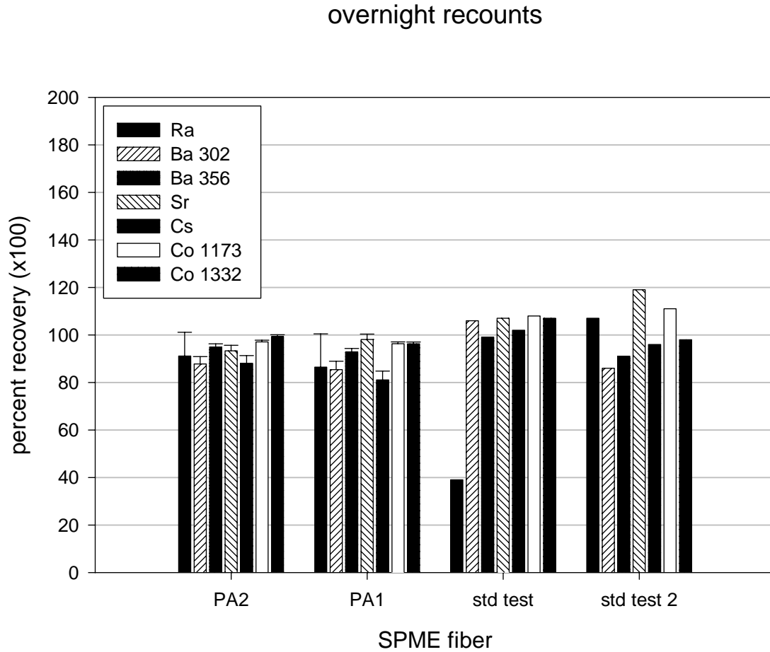
Figure 7 Overnight counting results of the polyacrylate (PA) SPME fibers that were exposed to low levels of radionuclides—in addition to duplicate analyses of the control solution. The numbers after the chemical symbols in the legend represent the gamma X-ray energies (in keV) that were counted. For Ra, Sr and Cs, only one gamma X-ray energy was used for counting.
