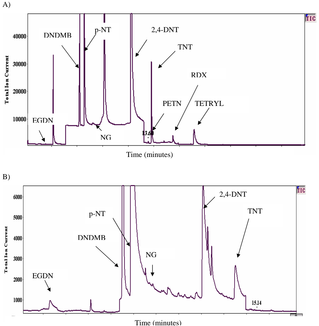
Figure 9 The results from the selective ion monitoring analyses of a) direct solvent injection of the HE standard (1 \mu\text{l} of 50 \text{mg L}^{-1} HE standard in acetone) showing the presence of the thermally-unstable RDX and NG-type compounds and b) the results of a 500 ng amount of (initially added) HE residue from one of the soil exposures.
