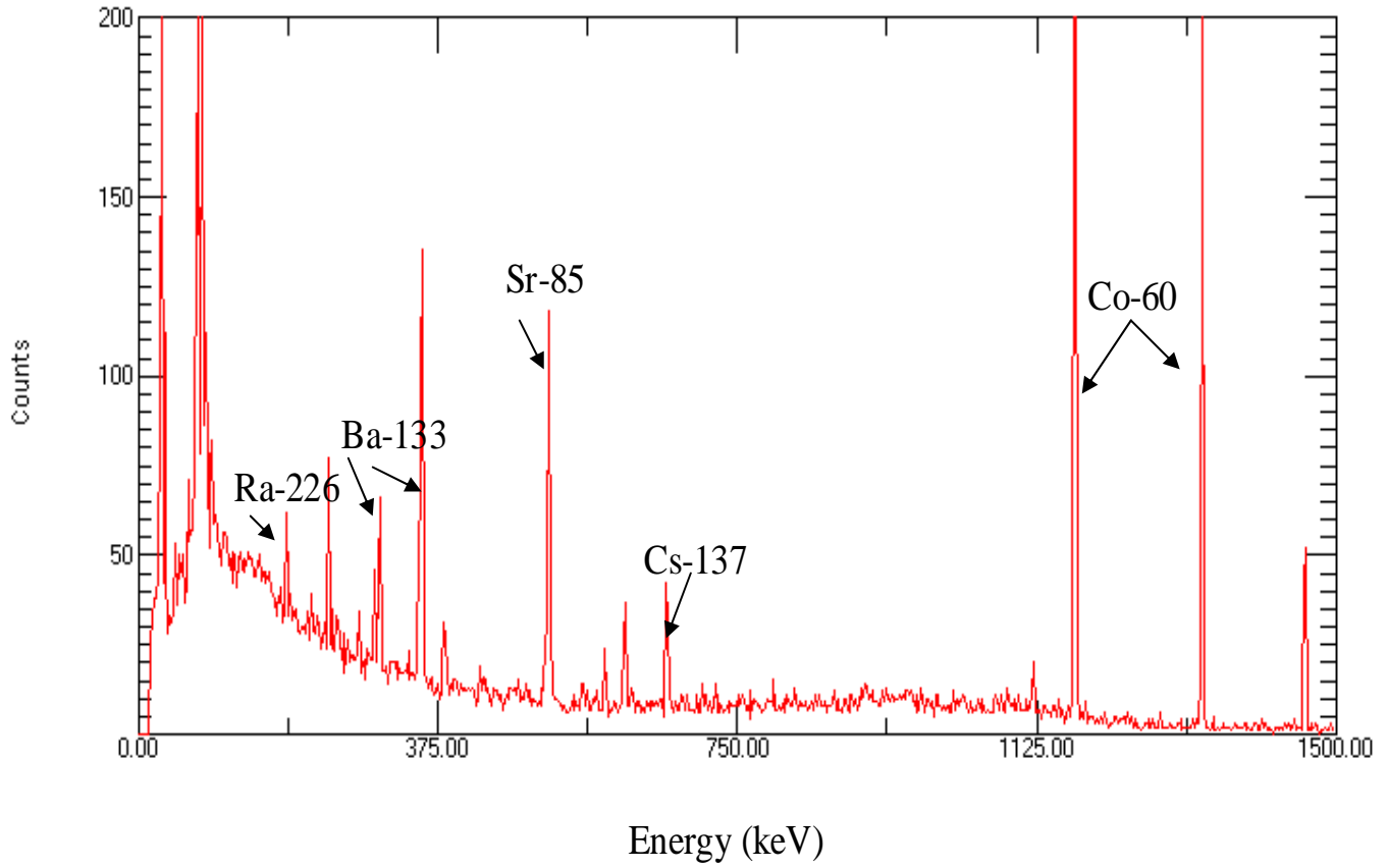
Figure 5 Gamma energy spectrum of the low level radionuclide solution after exposure to a CBX-PDMS SPME fiber.
