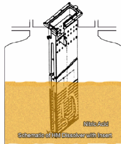
Figure 3: Dissolver with Mark XII Insert
