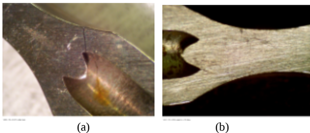
Fig. 13. Type 2 cracks observed in (a) as pinch welded and (b) end-milled test samples.
