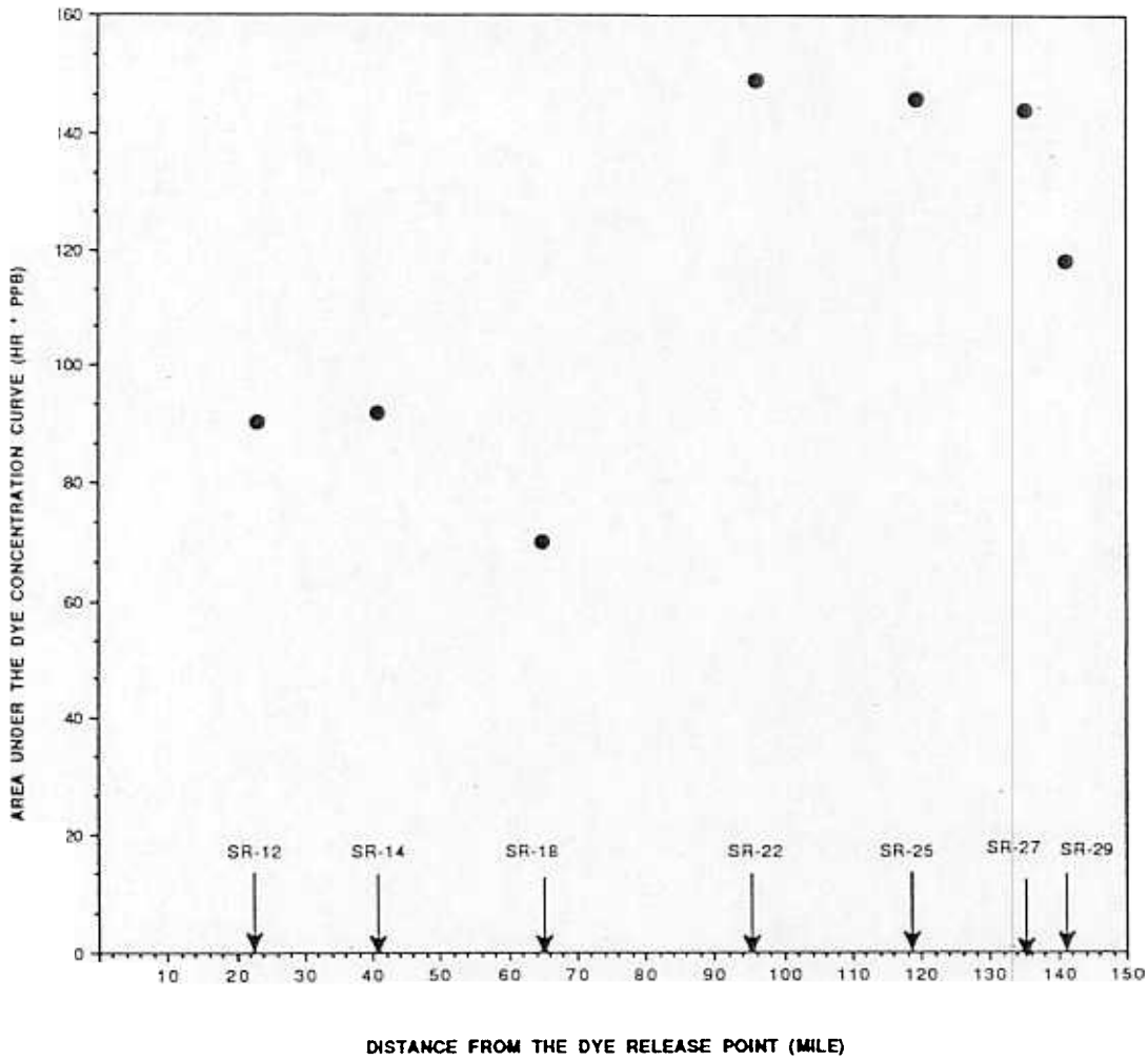
Figure 7 Area under the Measured Dye Concentration Curves (US EPA 1990 Dye Tracer Study)
