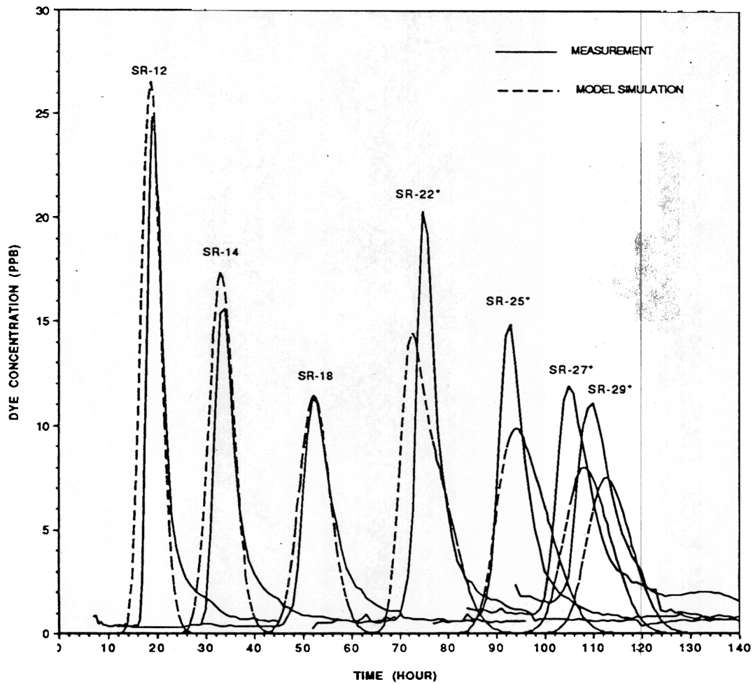
Figure 9 WASP5 Simulation for US EPA 1991 Dye Tracer Study
