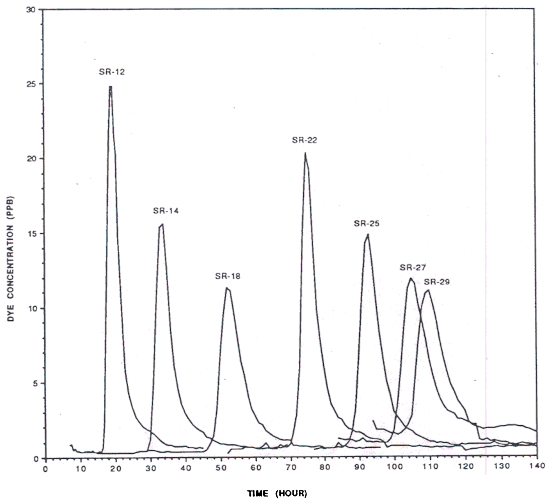
Figure 6 Measured Dye Tracer Profiles at the Sampling Stations (US EPA 1991 Dye Tracer Study)
