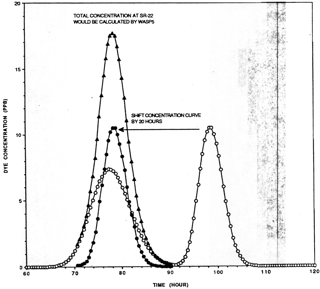
Figure 11 Total Concentrations at Poor Robin Landing (SR-22) Would be Calculated by WASP5 If the Input of the Additional Dye Release Time Were at 16:00 on 9/7/91
