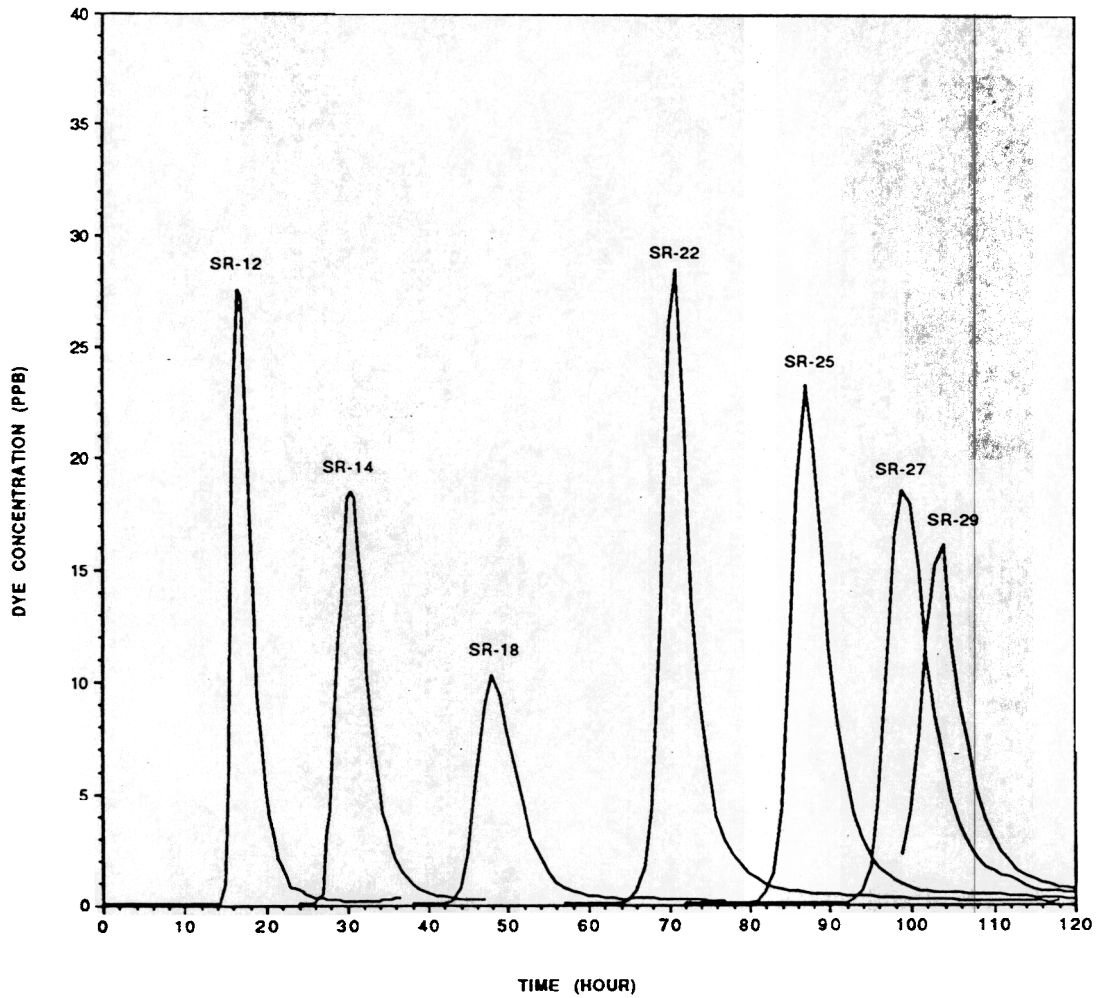
Figure 5 Measured Dye Tracer Profiles at the Sampling Stations (US EPA 1990 Dye Tracer Study)
