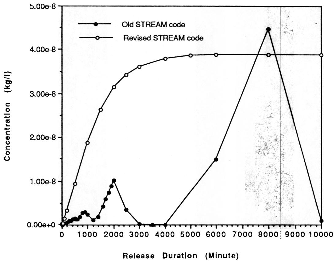
Figure 1 Calculated Concentrations at Highway 301 (Constant Release Rate of 0.5 kg/min from H-Area)
