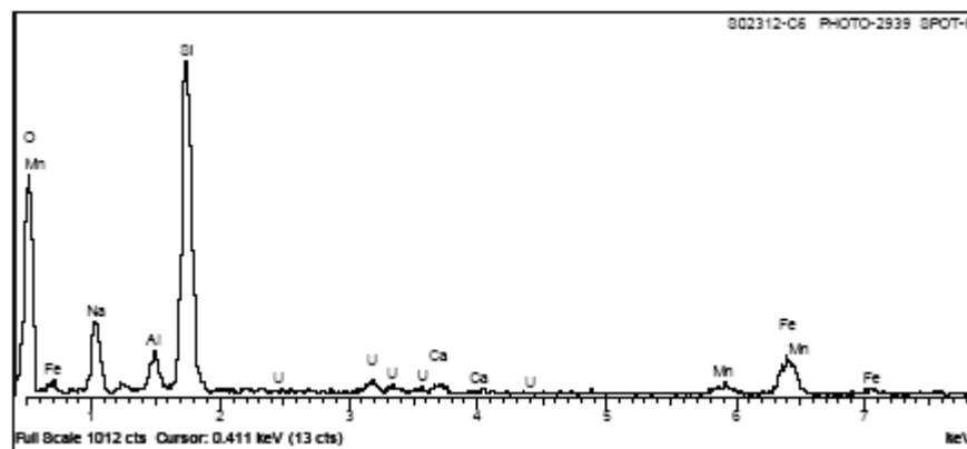
Fig. 3. X-Ray Fluorescence Spectra of Raster Scan of Spot 6 in Fig. 2 for DWPF Pour Stream Glass Sample S02312
