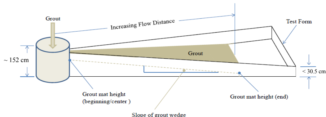
Figure 1. Schematic drawing illustrating the long-radius test configuration.
