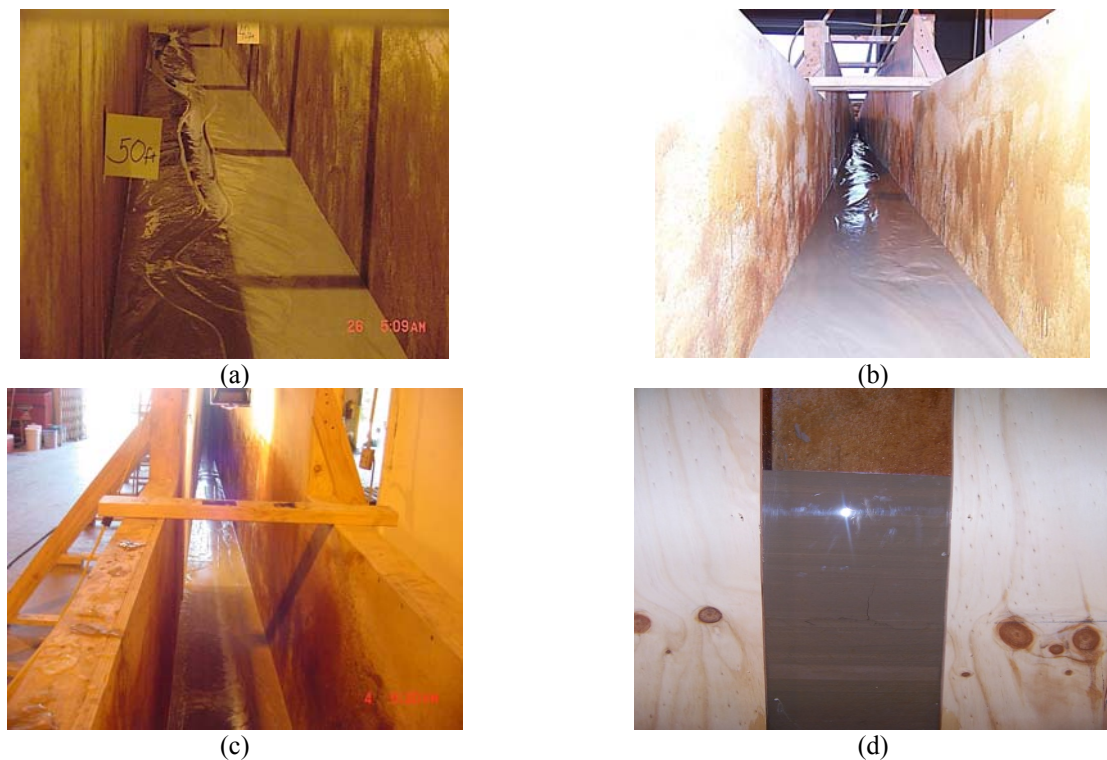
Figure 5. Grout flow in the test stand. (a) Narrow meandering channel and rippled surface characteristic of the test T11. (b) Medium meandering channel characteristic of the T10 surface. (c) Straighter flow channel characteristic of the T12 surface. (d) Striations in the flow as viewed through the Plexiglas® window about 61cm from the discharge point.
