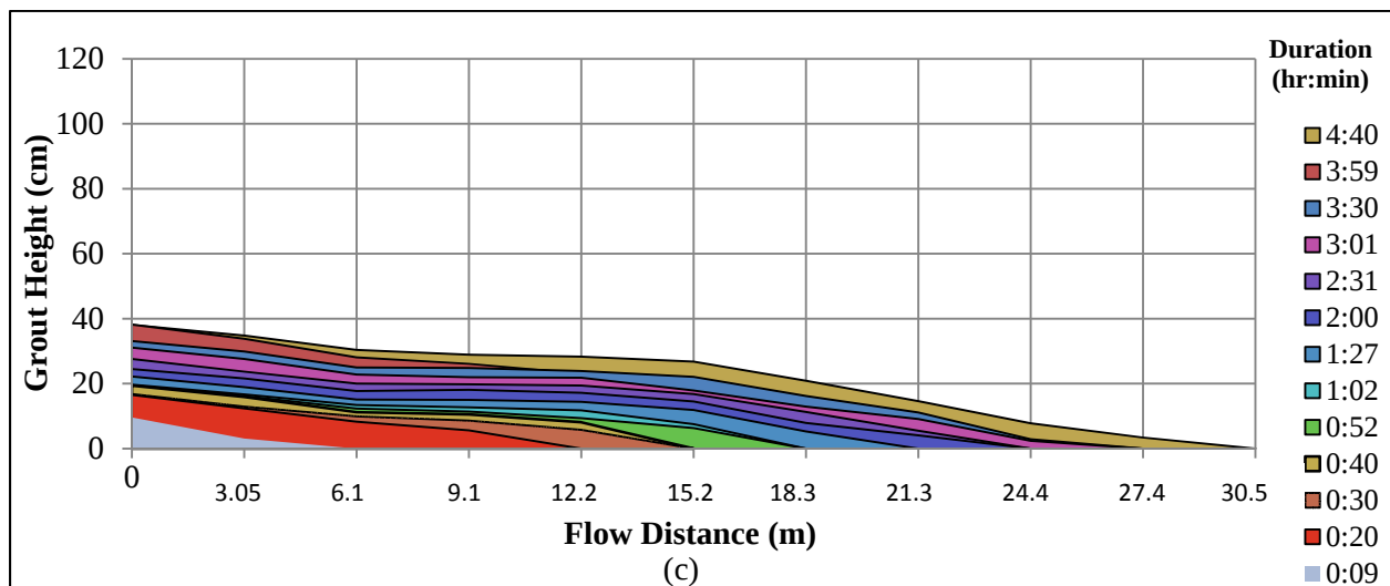
Figure 6. Surface profiles for long-radius pours: (a) T10-CC1, (b) T11-CC2 and (c) T12-CC1A
